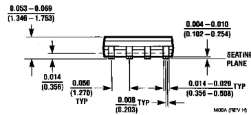
S.O. Package (M) Order Number LM78L05ACM, LM78L12ACM or LM78L15ACM NS Package Number M08A
