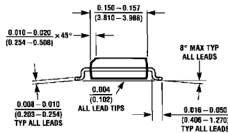
S.O. Package (M) Order Number LM78L05ACM, LM78L12ACM or LM78L15ACM NS Package Number M08A
