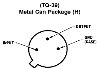
Bottom View Order Number LM78L05ACH, LM78L12ACH or LM78L15ACH See NS Package Number H03A
