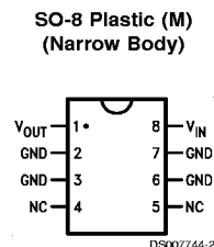
Top View Order Number LM78L05ACM, LM78L12ACM or LM78L15ACM See NS Package Number M08A
